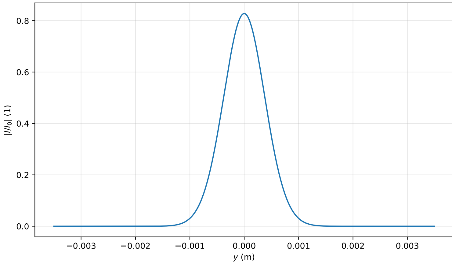
Intensity profile I(x=0, y, z=1.035)/I_0 , \text{Pin}=0.1\text{Pcr} , artificial time
